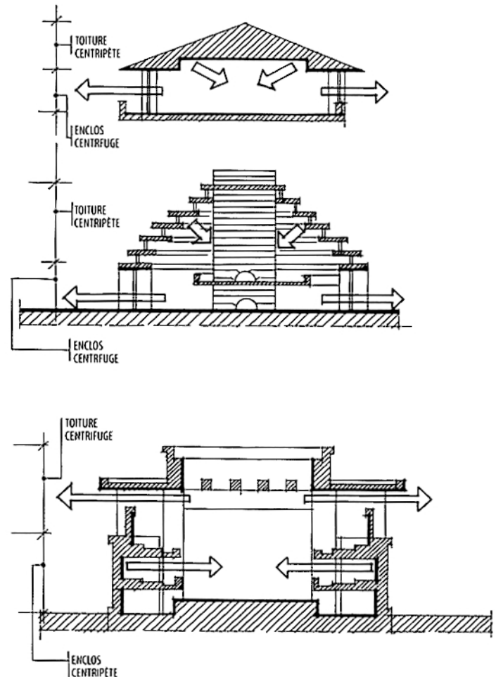
FIG. B-32 : Diagramme comparatif : Robie House, Wingspread House, Unity Temple.
